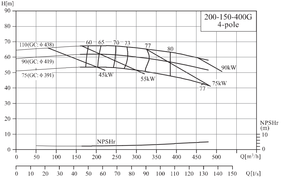
NIS/NISF200-150-400G
