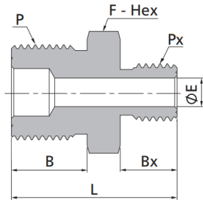
Male Metric Threads
