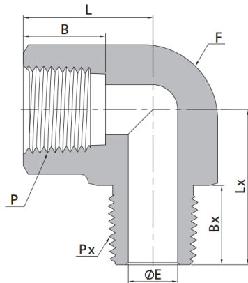
Female NPT Threads to Male NPT Thread
