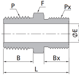
Male NPT Threads to Male Metric Threads
