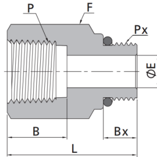
Female NPT Threads to Male SAE/MS Threads
