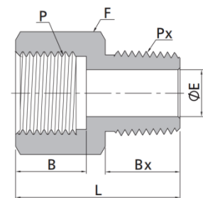
Female ISO Parallel Threads to Male NPT Threads
