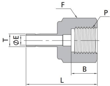
Metric Tube to ISO Parallel Thread
