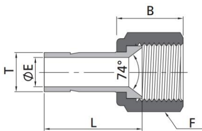
Fractional Tube to Flared
