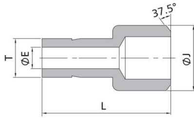
Fractional Tube to Pipe Weld
