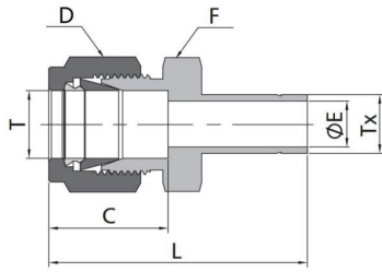
Metric Tube to Fractional Tube
