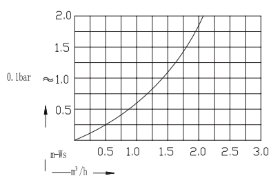
普通上下集散 1" top and bottom distributor
