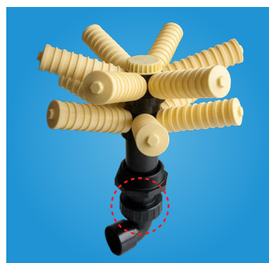
(UNION CONNECT)
